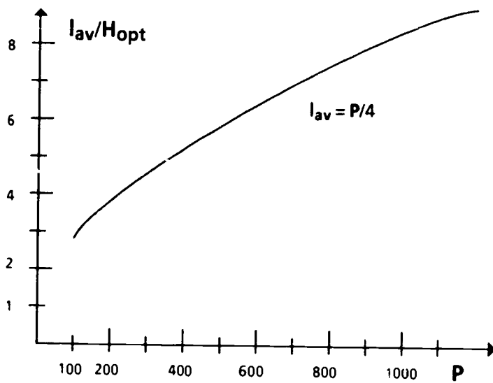
Graph A1 I_{av}/H_{opt} vs. P
