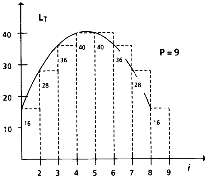
Graph A3 Link traffic vs. link position
