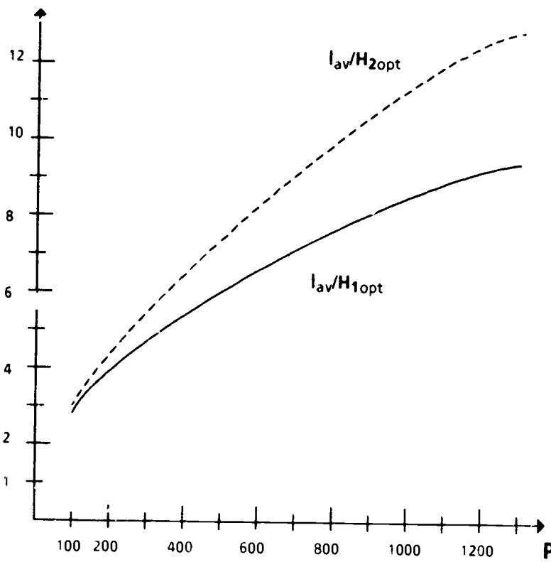
Graph A2 I_{av}/H_{1opt} and I_{av}/H_{2opt} vs. P
