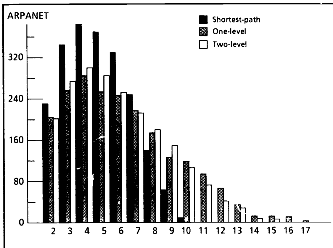
Shortest path vs one- and two-level Cartesian routing
