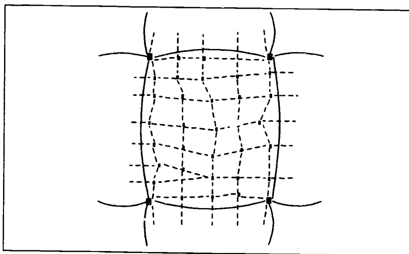
Fig. 10 Portion of level (0) and level (1) connection grids
